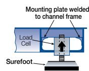
RoughDeck scale corner
